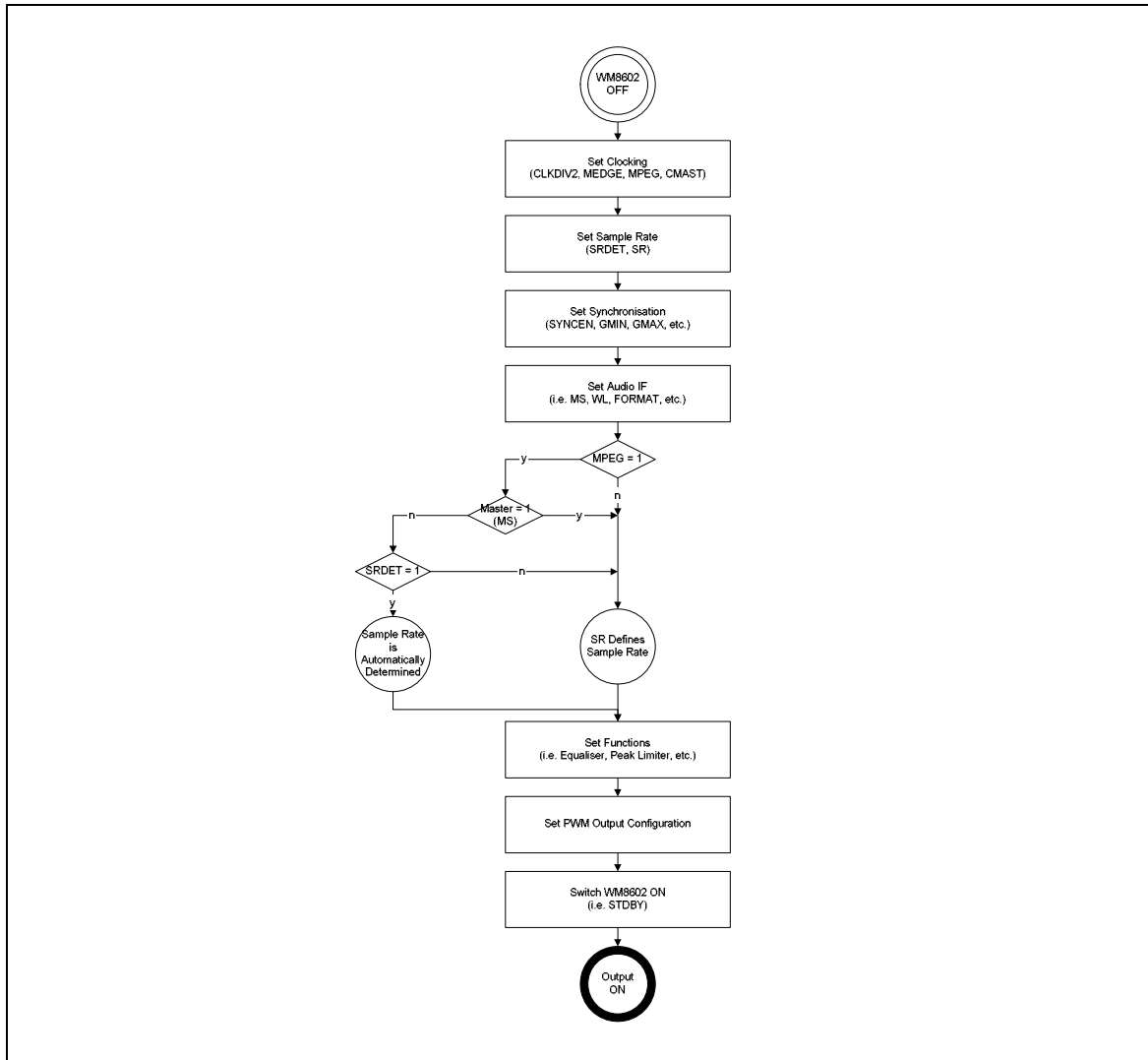
Figure 36 WM8602 Start-up
