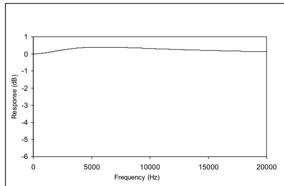
Figure 35 De-Emphasis Error (48kHz)
