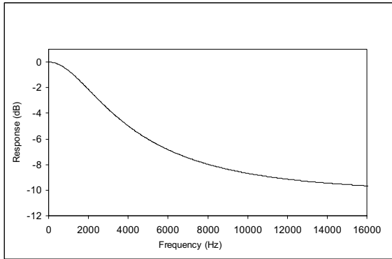
Figure 30 De-Emphasis Frequency Response (32kHz)
