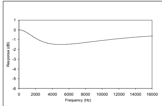
Figure 31 De-Emphasis Error (32kHz)
