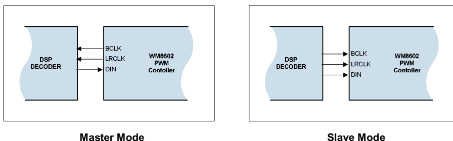
Figure 8 Operation Mode
