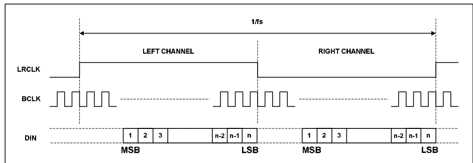
Figure 10 Right Justified Mode Timing Diagram
