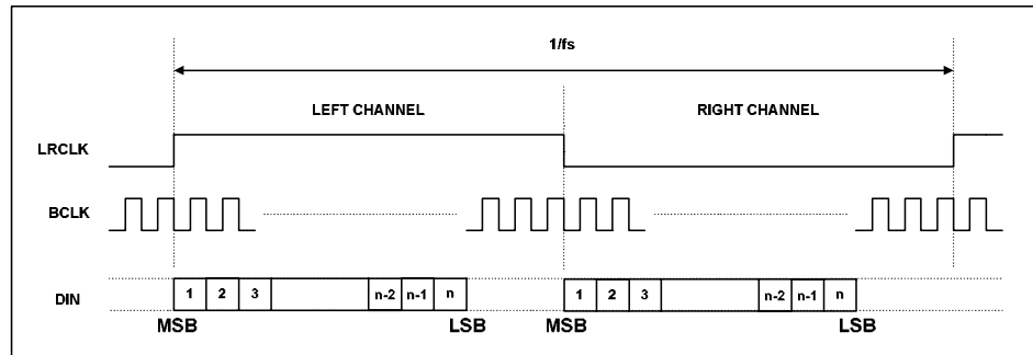
Figure 9 Left Justified Mode Timing Diagram
