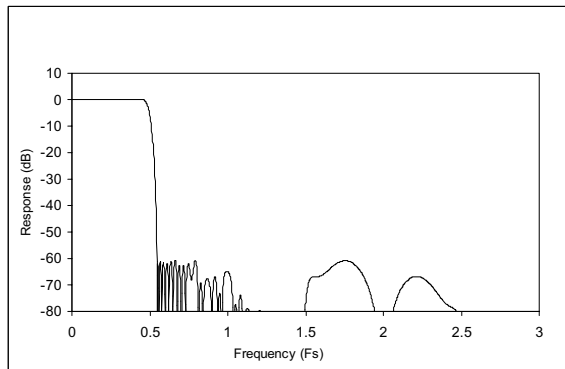
Figure 26 Digital Filter Frequency Response – 44.1, 48 and 96kHz
