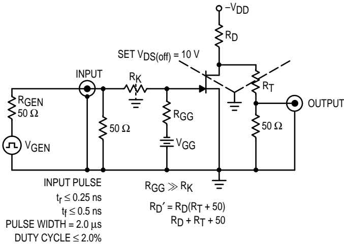
Figure 5. Switching Time Test Circuit
