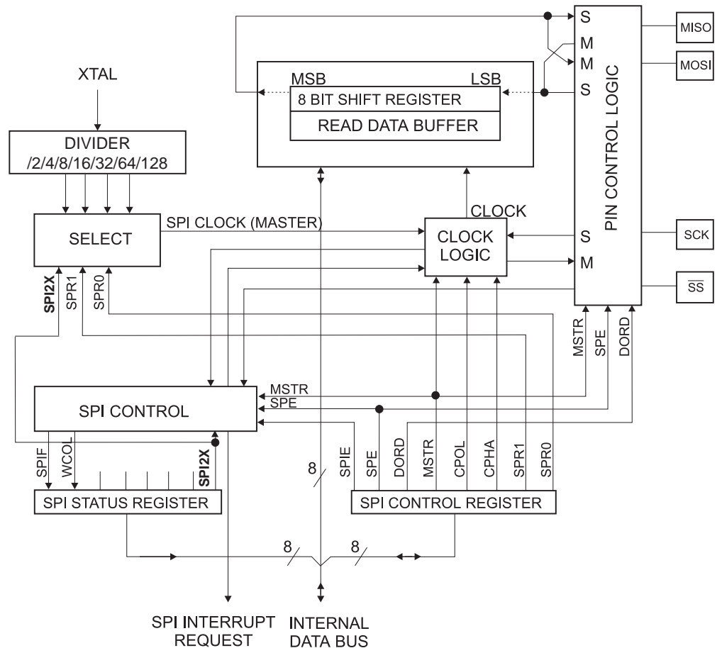
Figure 75. SPI 方框图
