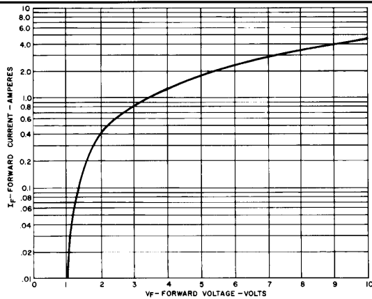
Fig. 3. Forward Voltage vs. Forward Current ST1053
