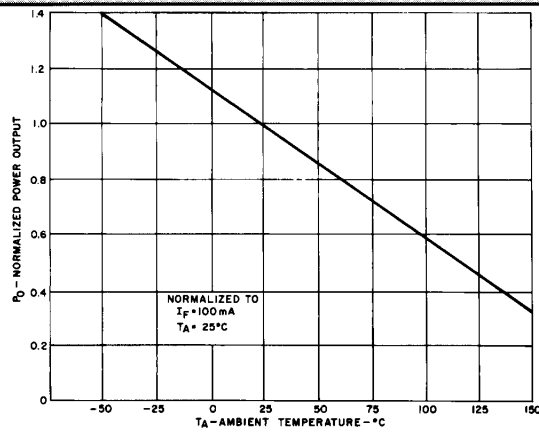
Fig. 2. Power Output vs. Temperature ST1057
