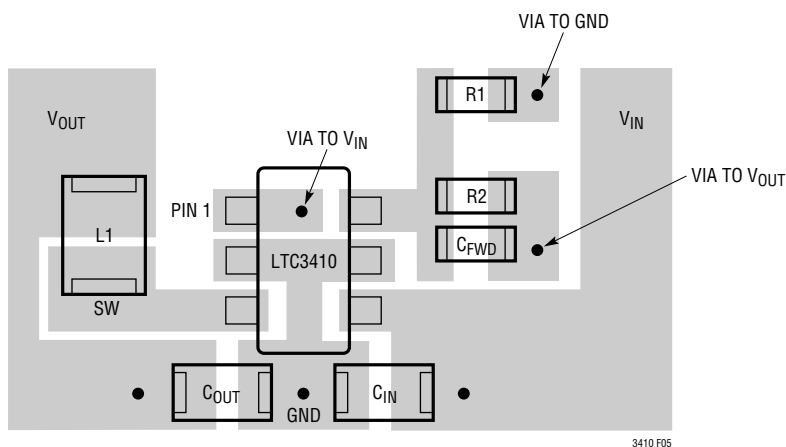
Figure 5. LTC3410 Suggested Layout
