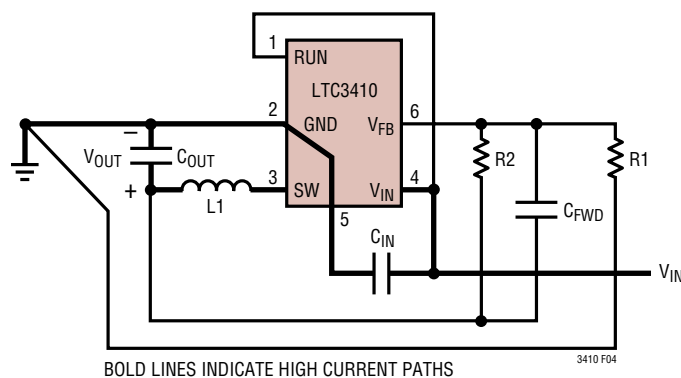
Figure 4. LTC3410 Layout Diagram
