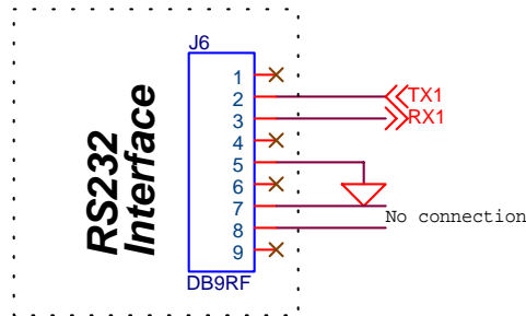
Figure 5. RS232C connector
