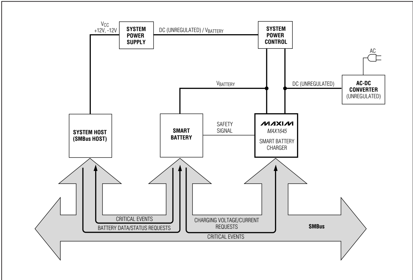
Figure 10. Typical Single Smart Battery System
