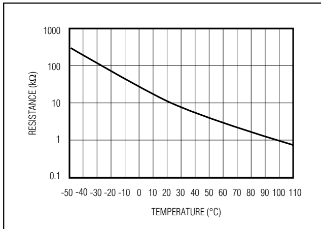
Figure 9. Typical Thermistor Characteristics
