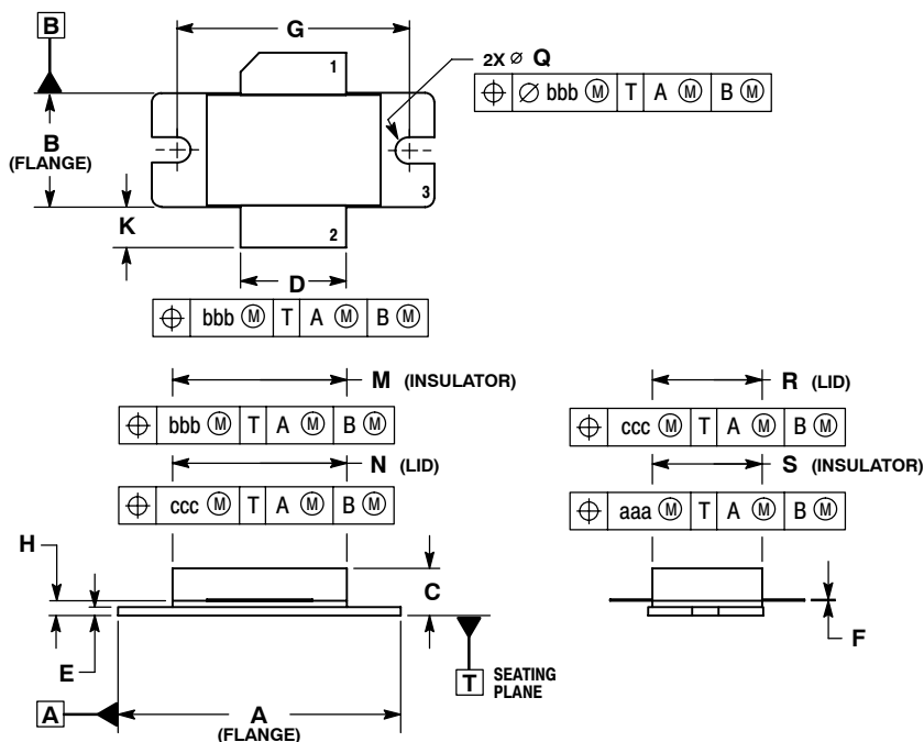
CASE 465B-03 ISSUE B NI-880 MRF5S21130HR3
