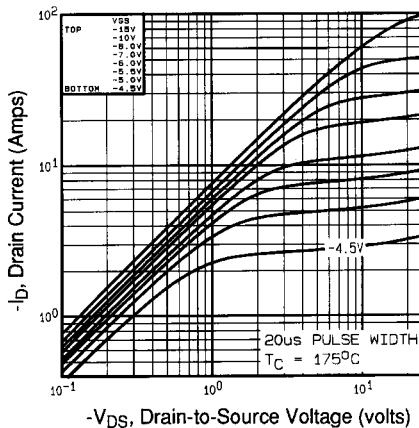
Fig 2. Typical Output Characteristics, T_C = 175^\circ\text{C}
