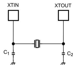
(2) Low-frequency Oscillation
