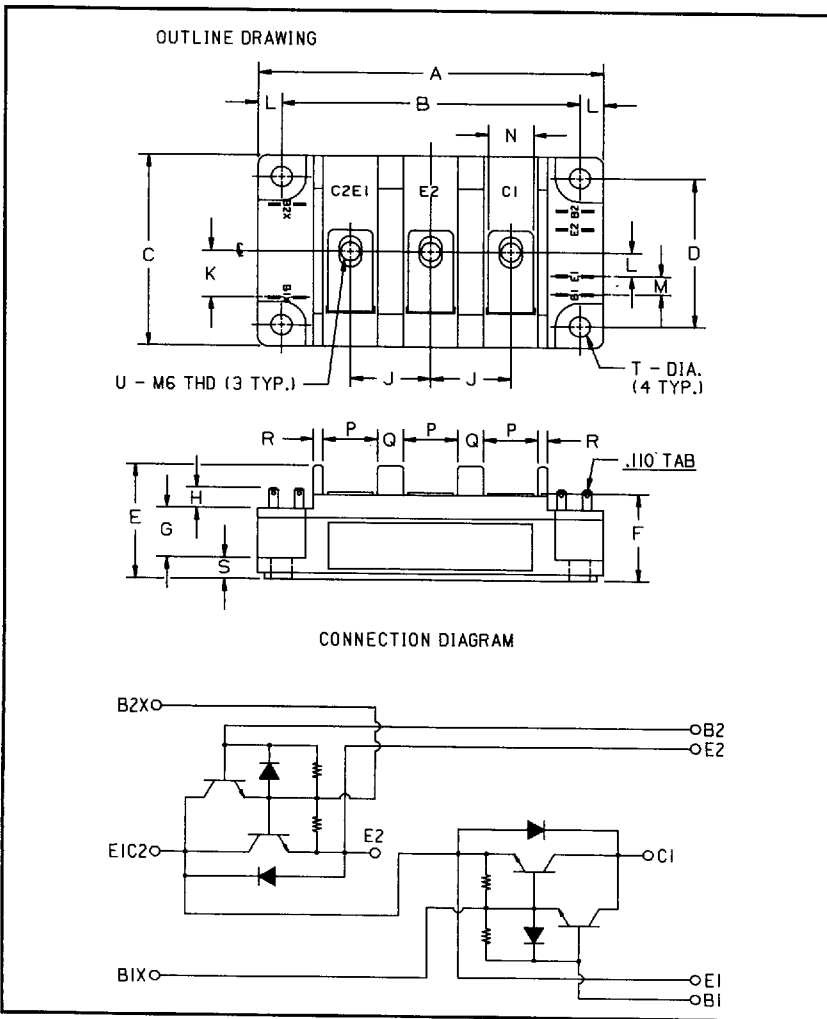
Outline Drawing
