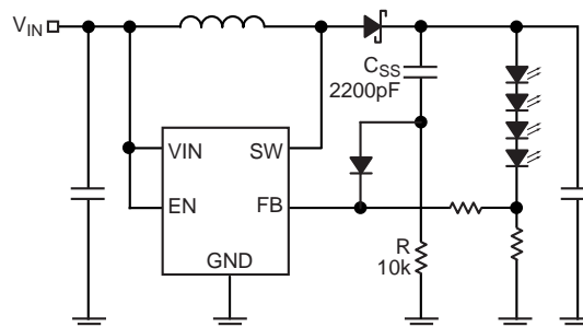
Figure 5. Soft-Start Circuit
