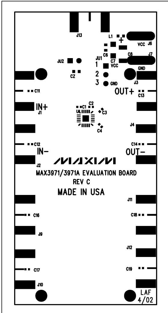
Figure 2. MAX3971/MAX3971A EV Kit Component Placement Guide-Component Side
