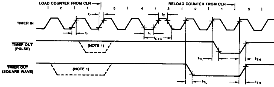
Timer Output Waveform Countdown from 5 to 1
