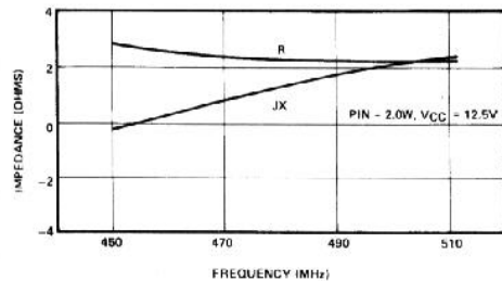
COLLECTOR LOAD IMPEDANCE VS FREQUENCY
