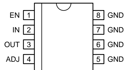
MIC37102 (Adjustable) SOIC-8 (M)
