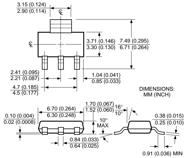
SOT-223 (S)
