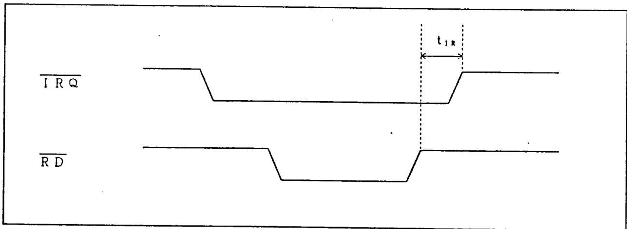
Figure 5.2 \overline{\text{IRQ}} timing
