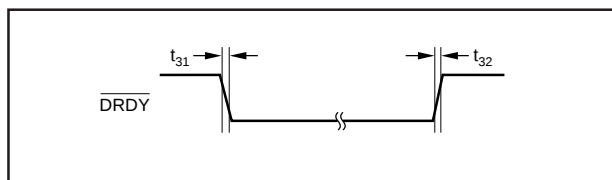
FIGURE 21. \overline{DRDY} Rise and Fall Time.
