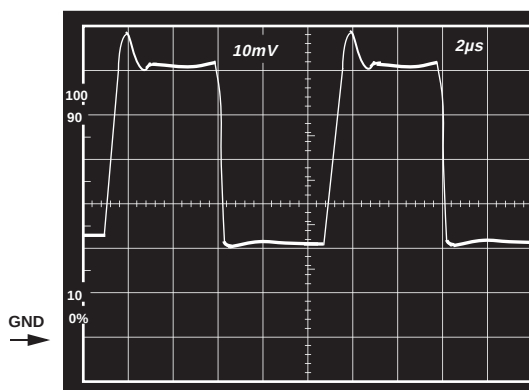
Figure 36. V_S = +5\text{ V} , 0\text{ V} ; Gain of Two Inverter Response to 20\text{ mV} Step, Centered 20\text{ mV} Below Ground, R_L = 10\text{ k}\Omega
