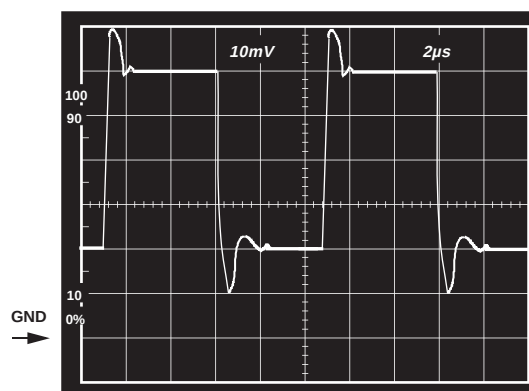
Figure 35. V_S = +5\text{ V} , 0\text{ V} ; Unity Gain Follower Response, to 40\text{ mV} Step Centered 40\text{ mV} Above Ground, R_L = 10\text{ k}\Omega
