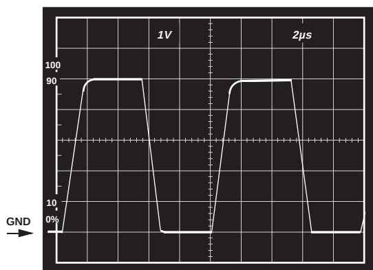
Figure 37. V_S = +5\text{ V}, 0\text{ V} ; Gain of Two Inverter Response to 2.5\text{ V} Step Centered -1.25\text{ V} Below Ground, R_L = 10\text{ k}\Omega
