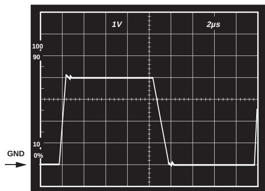
Figure 31. V_S = +5\text{ V} , 0\text{ V} ; Unity Gain Follower Response to 0\text{ V} to 4\text{ V} Step
