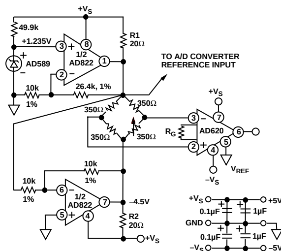
Figure 47. Low Dropout Bipolar Bridge Driver
