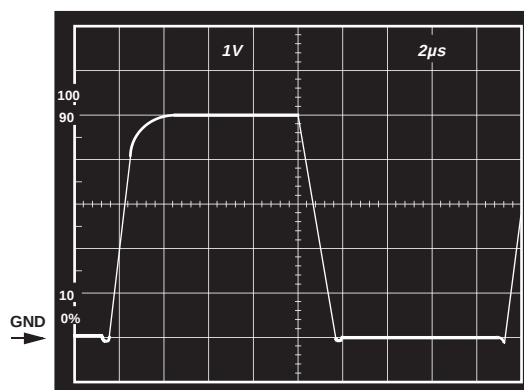
Figure 34. V_S = +5\text{ V} , 0\text{ V} ; Unity Gain Follower Response to 0\text{ V} to 5\text{ V} Step
