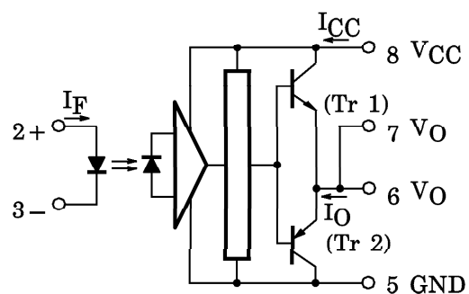
SCHMATIC
