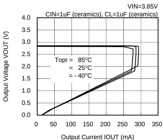
XC6401(2.85V)
