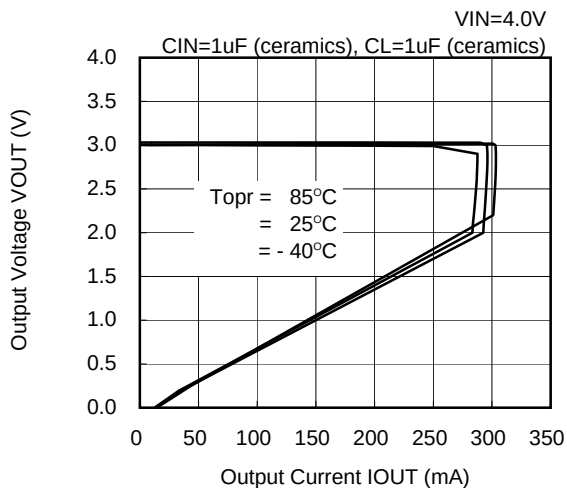
XC6401(3.0V)
