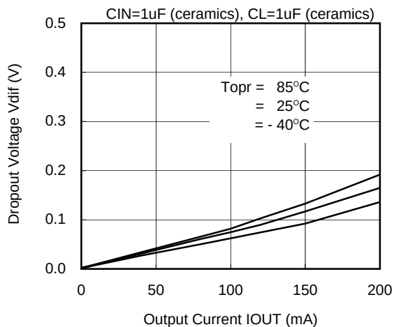
XC6401(5.0V)
