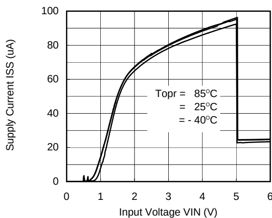
XC6401(5.0V)
