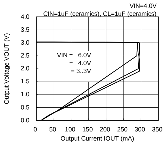
XC6401(3.0V)
