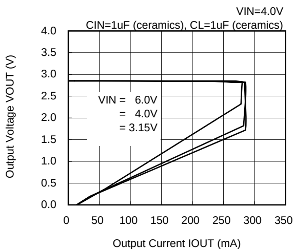
XC6401(2.85V)
