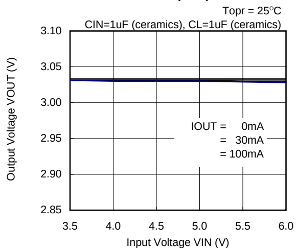
XC6401(3.0V)
