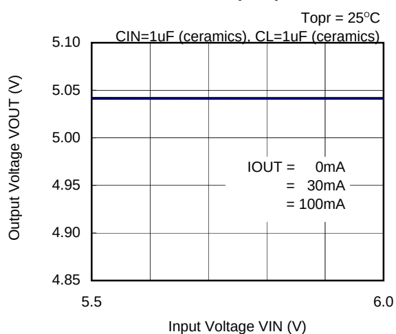
XC6401(5.0V)
