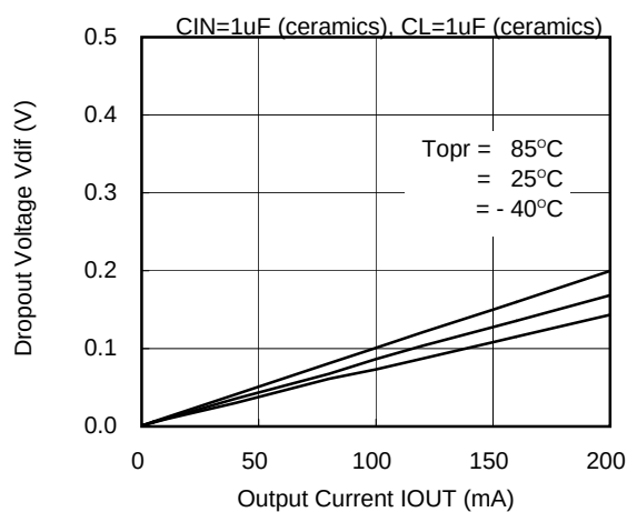
XC6401(2.85V)
