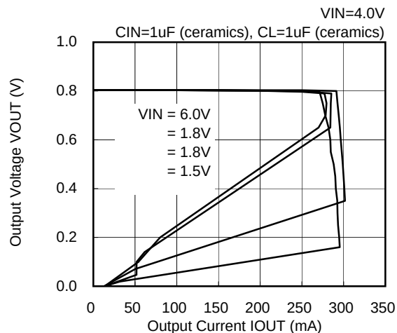
XC6401(0.8V)
