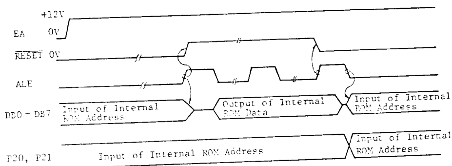
Fig.7 Timing of Reading Internal Program Memory
