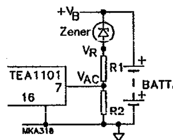
Fig.8 Basic circuit showing the use of a Zener diode.
