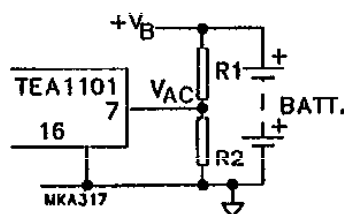
Fig.7 Basic circuit for direct battery sensing.
