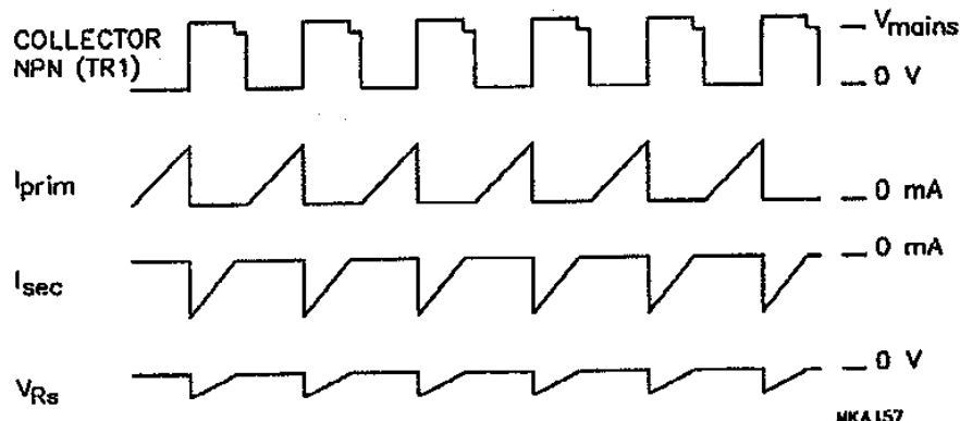
Fig.5 SMPS voltage and current waveforms.
