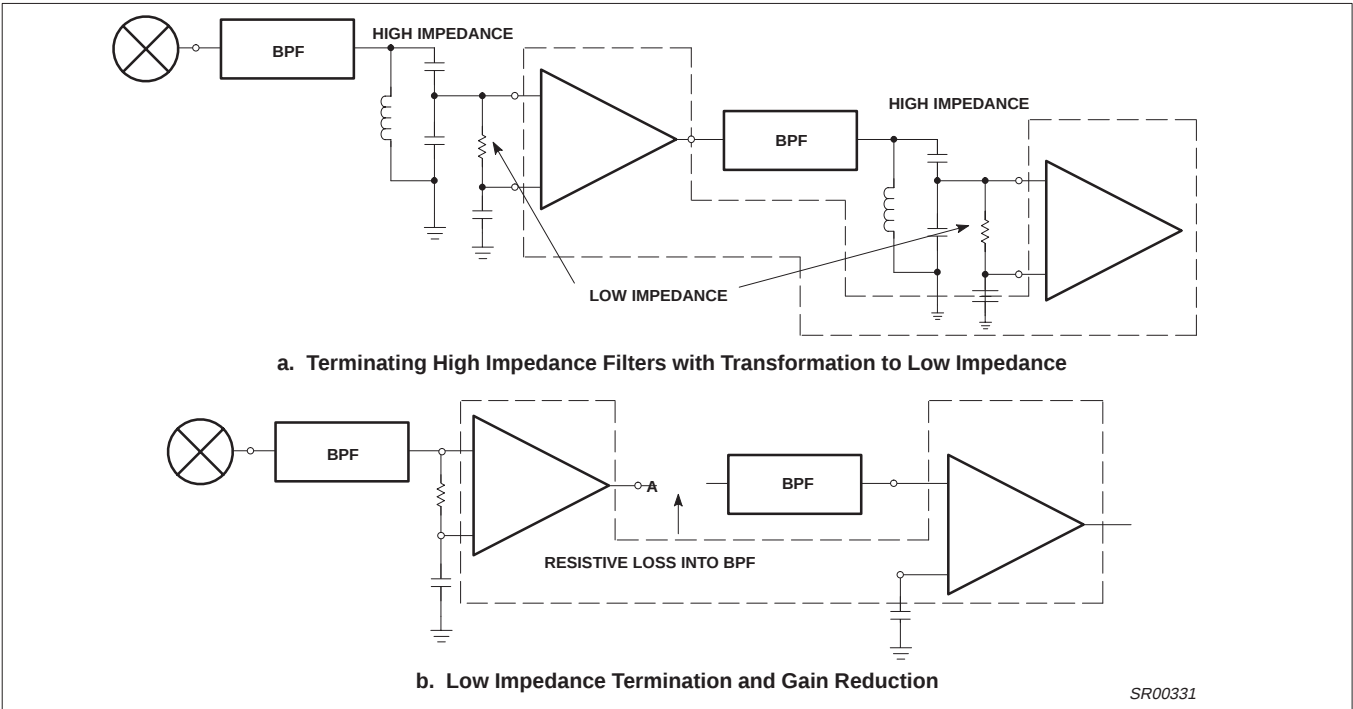
Figure 9. Practical Termination
