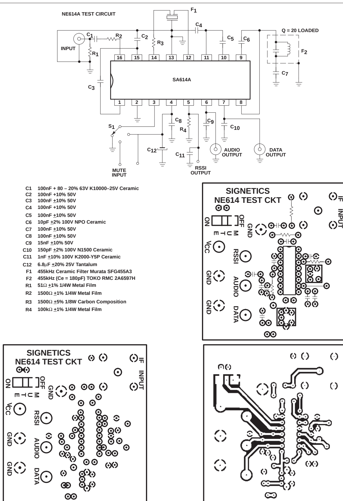
Figure 3. SA614A Test Circuit
