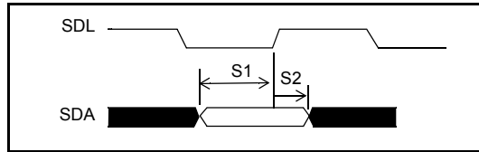
Figure 22 - I 2 C Input Setup Timing
