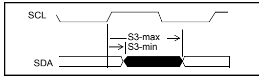
Figure 23 - I 2 C Output Delay Timing
