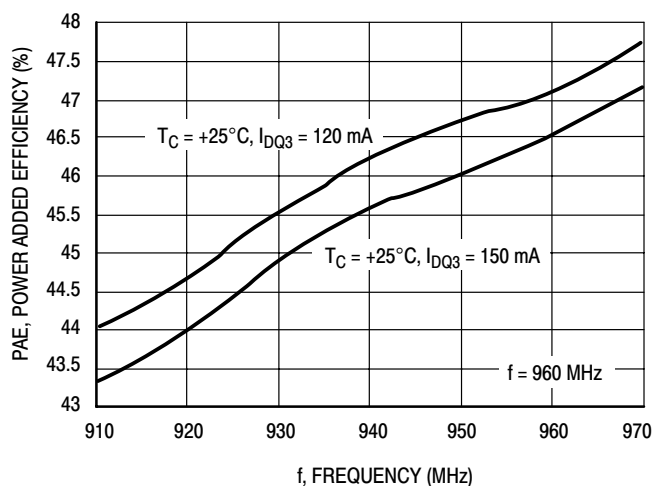
Figure 10. Power Added Efficiency versus Frequency Pout = 10 W
