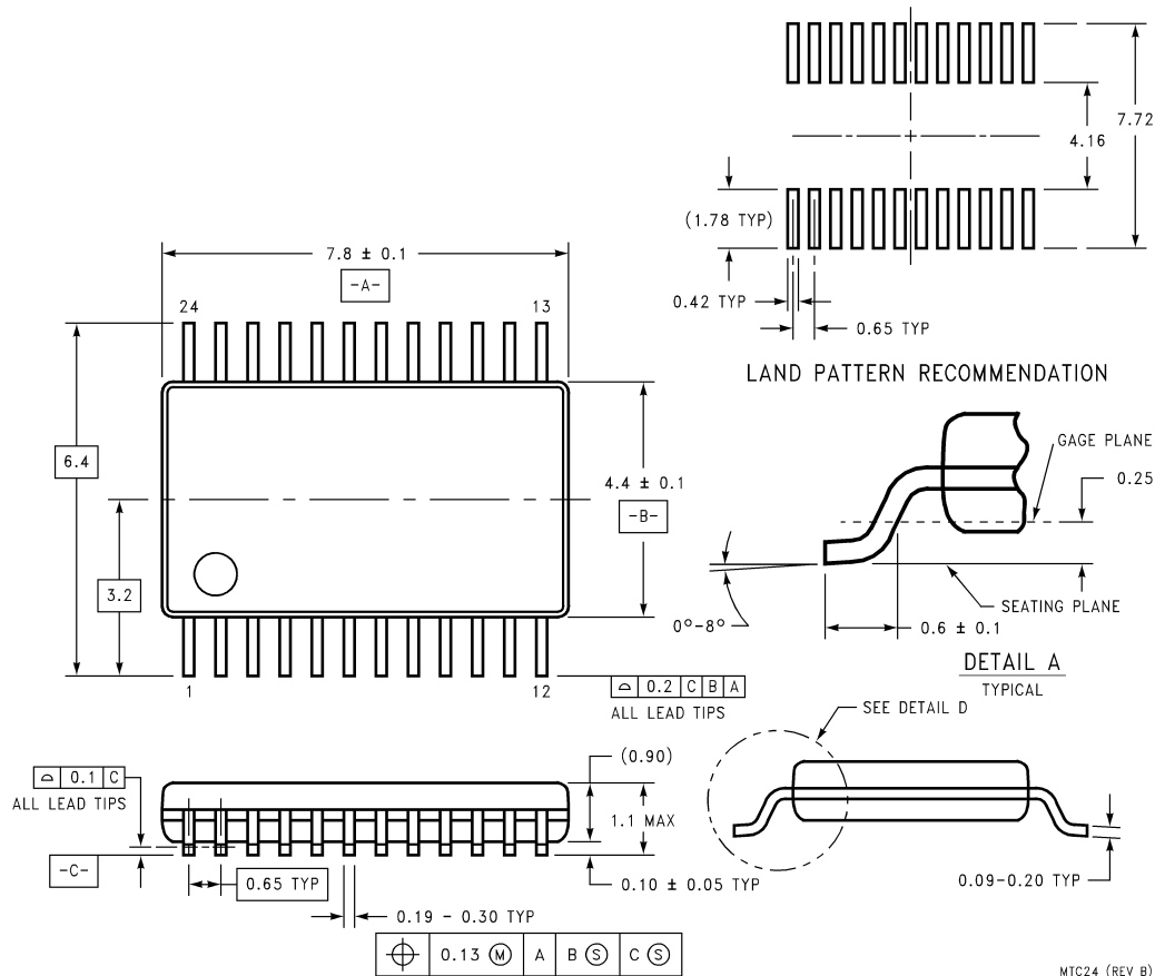
24-Lead TSSOP Order Number LM81CMT NS Package Number MTC24B
