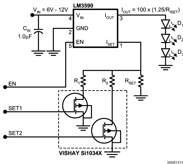
FIGURE 2. Example: R_1 = 15.8k\Omega , R_2 = 31.6k\Omega , R_{SET} = 31.6k\Omega
