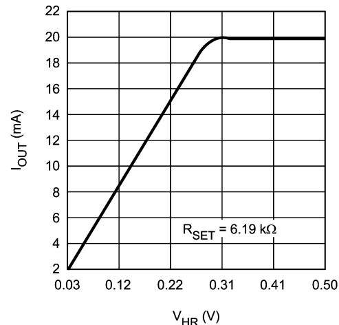
FIGURE 1. I_{OUT} vs V_{HR}
