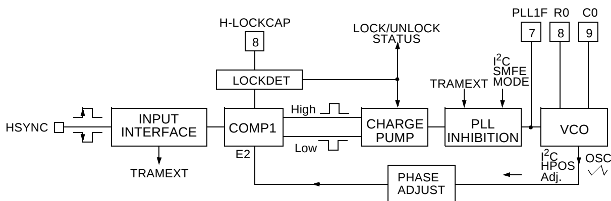
Figure 9. Block Diagram
