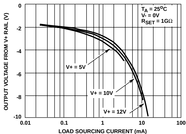
FIGURE 8. OUTPUT VOLTAGE vs SOURCING LOAD CURRENT
