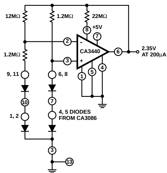
FIGURE 4. MICROPOWER BANDGAP REFERENCE
