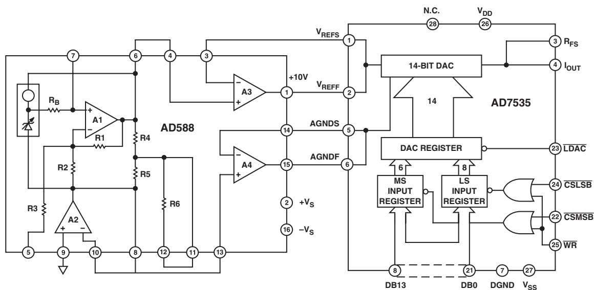
Figure 20. AD588/AD7535 Connections
