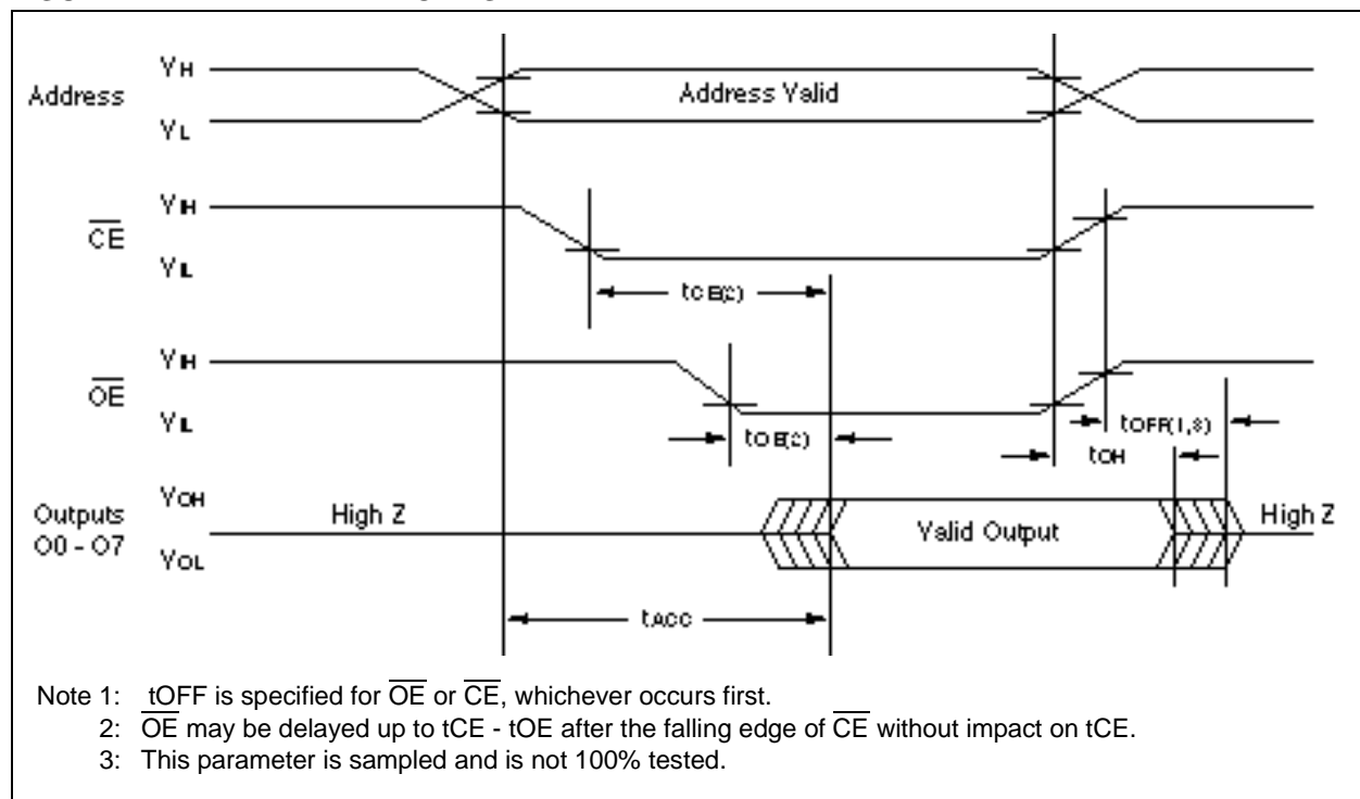
FIGURE 1-1: READ WAVEFORMS
