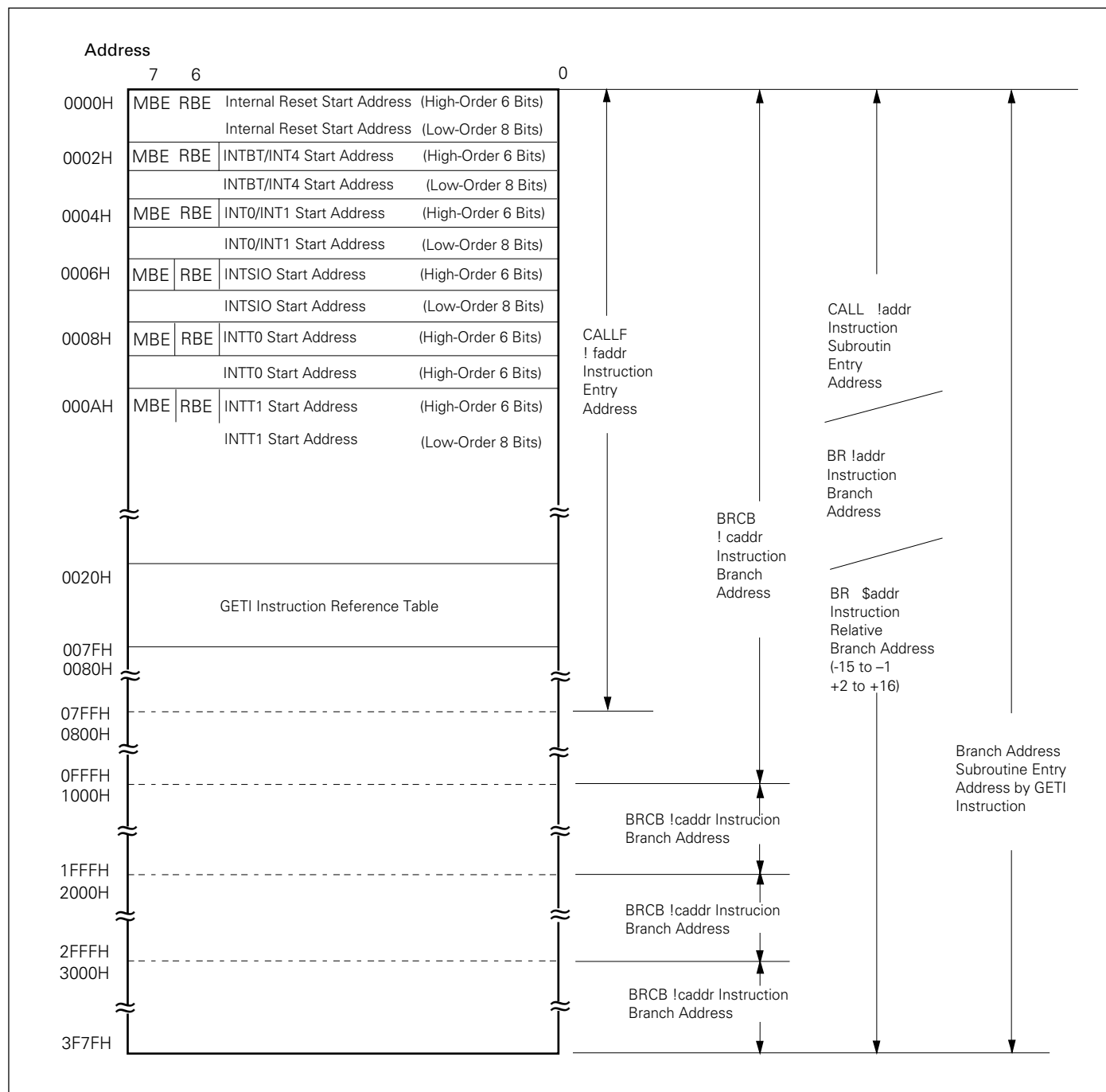
Figure 4-2 Program Memory Map ( \mu PD75116(A))
