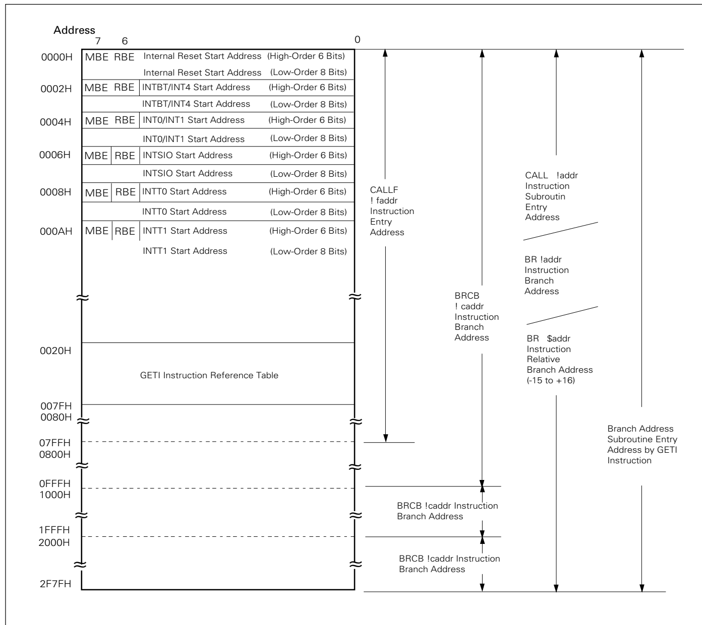
Figure 4-1 Program Memory Map ( \mu PD75112(A))
