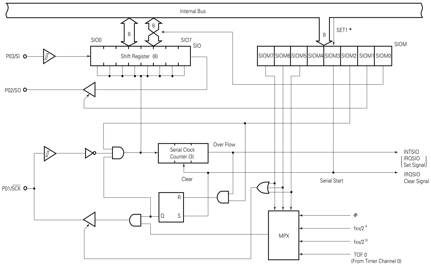
Figure 5-5 Block Diagram of Serial Interface
