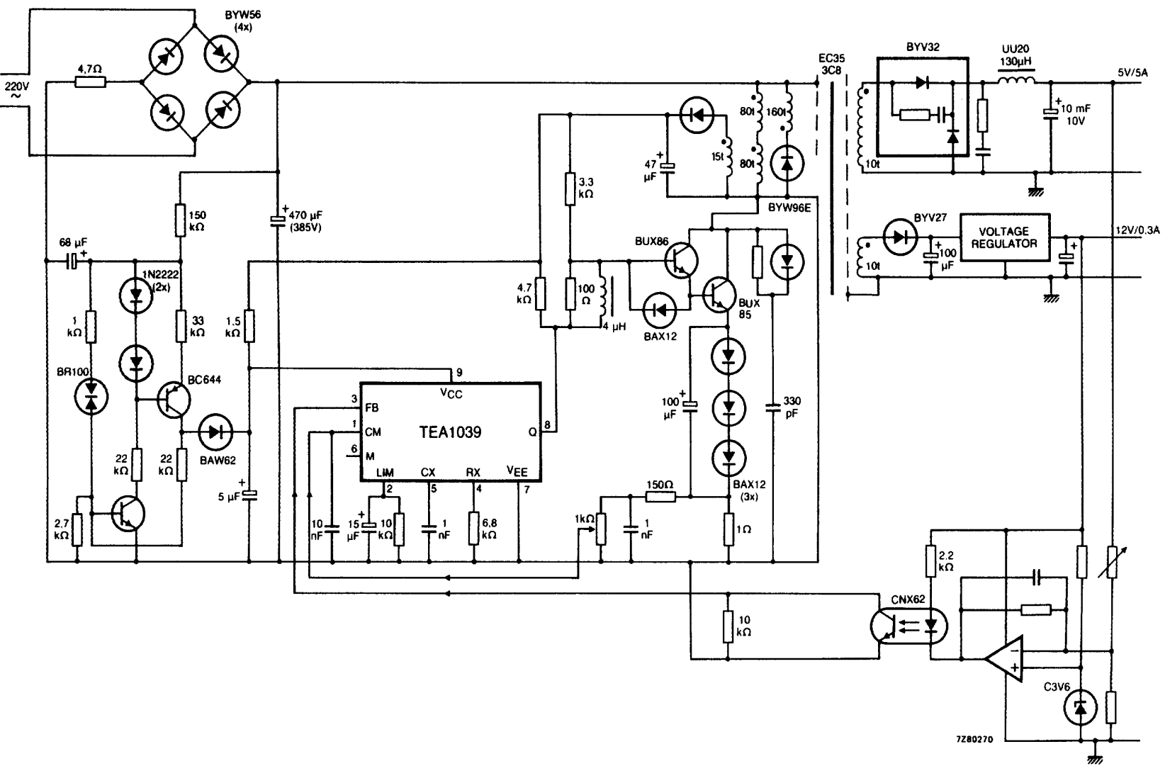
Fig.10 Typical application of the TEA1039 in a fixed-frequency, variable duty factor forward converter switched-mode power supply. An optocoupler CNX62 is used for voltage separation.
