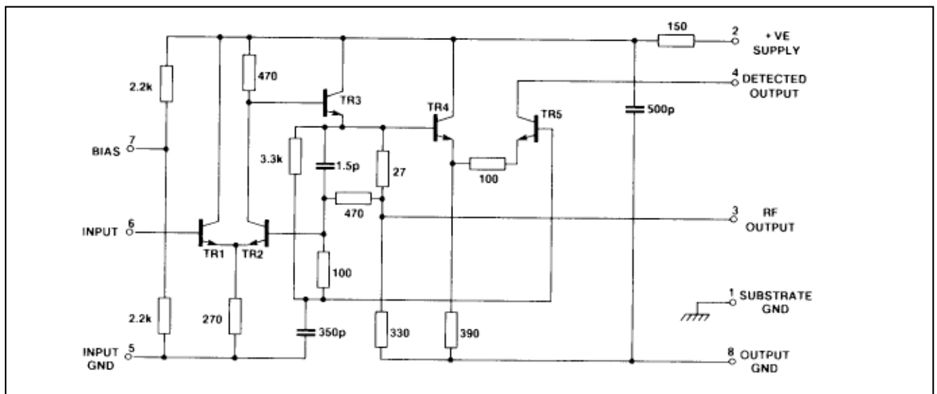
Fig.2 Circuit diagram
