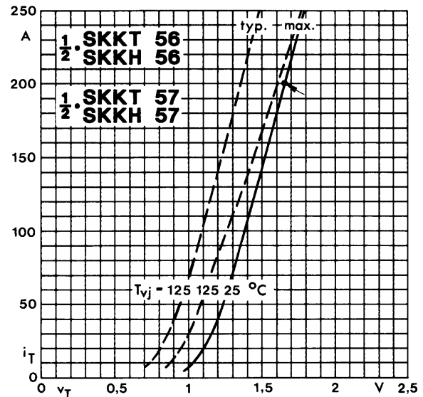
Fig. 8 On-state characteristics
