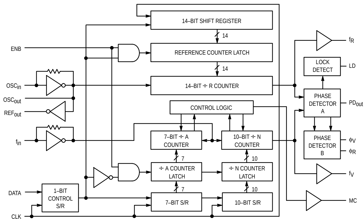
MC145158-2 BLOCK DIAGRAM
