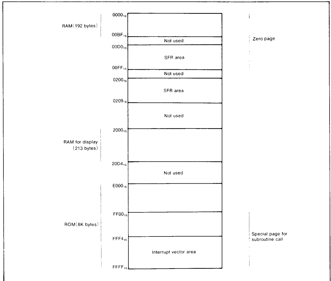
Fig. 1 Memory map
