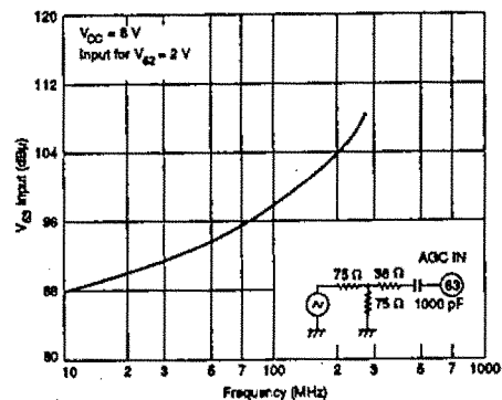
Figure 4. AGC frequency response
