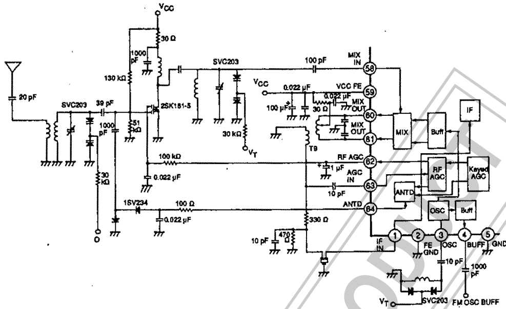
Figure 1. AGC stage
