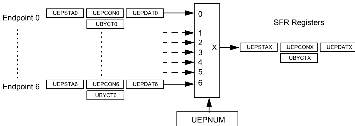
Figure 53. Endpoint Selection
