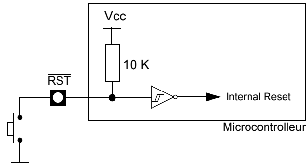
Figure 105. Reset Controlled by the User
