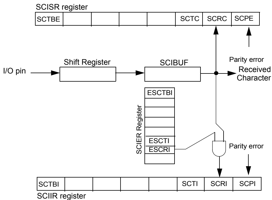
Figure 44. Character Reception Diagram
