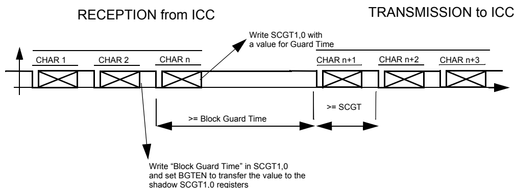
Figure 33. Guard Time and Block Guard Time counters
