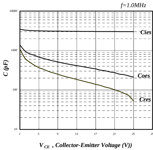
Fig 7. Typical Capacitance Characteristics
