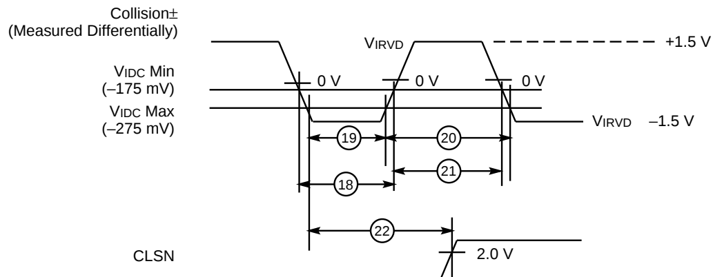
Collision± Input Pulse Width Timing
