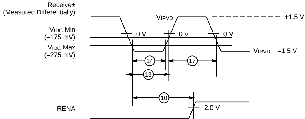
Receive± Input Pulse Width Timing
