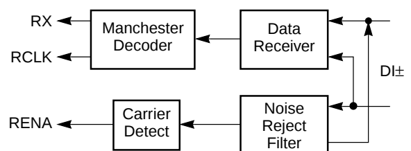
Figure 4. Receiver
