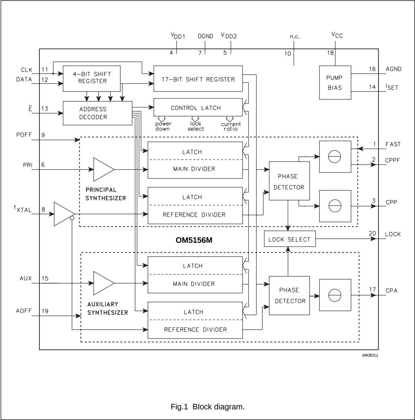
BLOCK DIAGRAM
