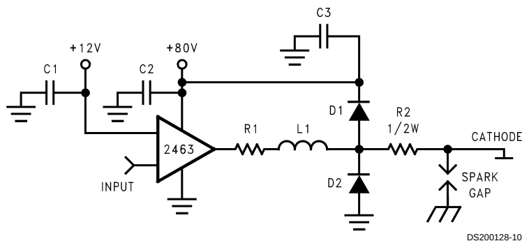
FIGURE 9. One Channel of the LM2463 with the Recommended Arc Protection Circuit
