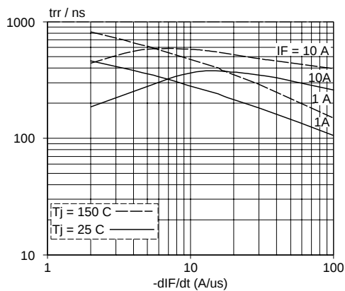
Fig.7. Maximum t_{rr} measured to 25% of I_{rrm} ; T_j = 25^\circ\text{C} and 150^\circ\text{C}
