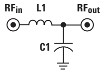
Figure 5. Low Pass Circuit Topology.
