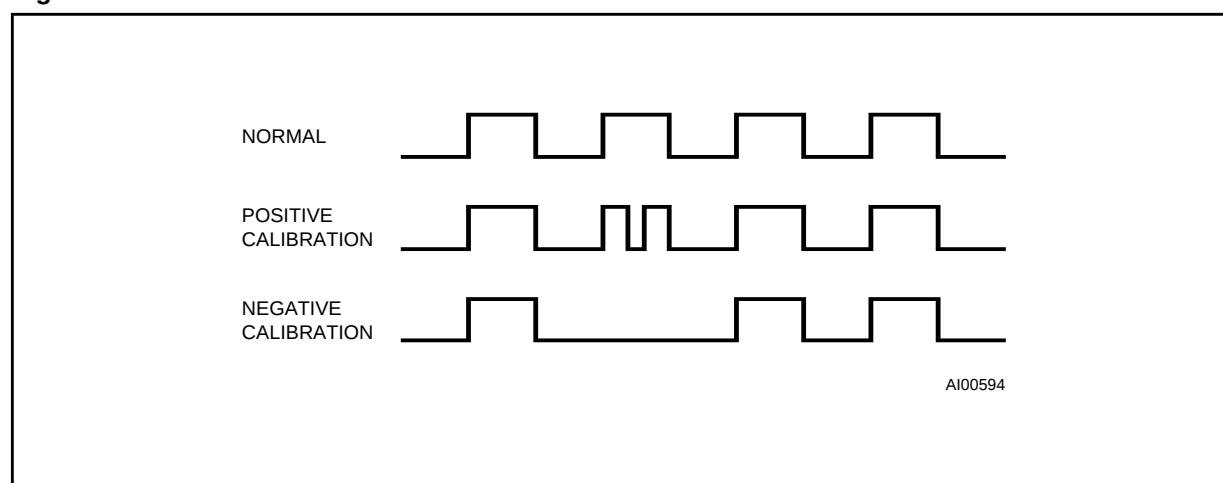
Figure 9. Clock Calibration
