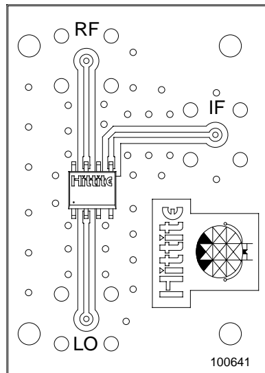
PC MOUNT SMA CONNECTORS IN THREE PLACES
