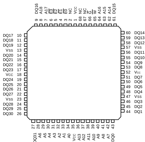
FIG. 1 PIN CONFIGURATIONS AND BLOCK DIAGRAM
