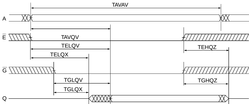
FIG. 5 READ CYCLE 2 - \bar{W} HIGH
