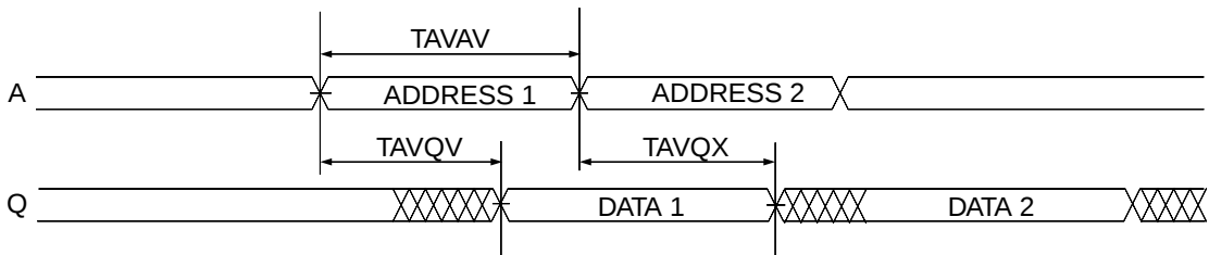
FIG. 4 READ CYCLE 1 - \bar{W} HIGH, \bar{G} , \bar{E} LOW
