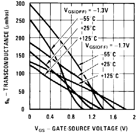
Transfer Characteristics
